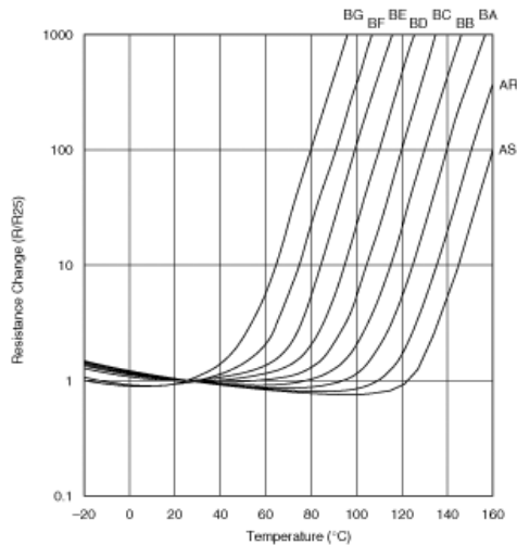
Resistance-Temperature Characteristics
