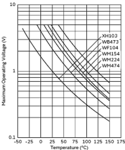
Maximum Operating Voltage Reduction Characteristics
