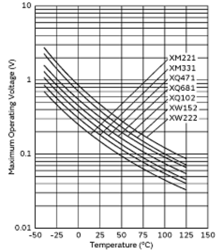
Maximum Operating Voltage Reduction Characteristics
