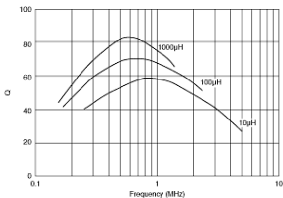
Q-Frequency Characteristics
