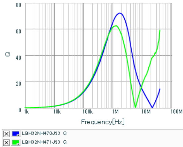
Q-Frequency Characteristics
