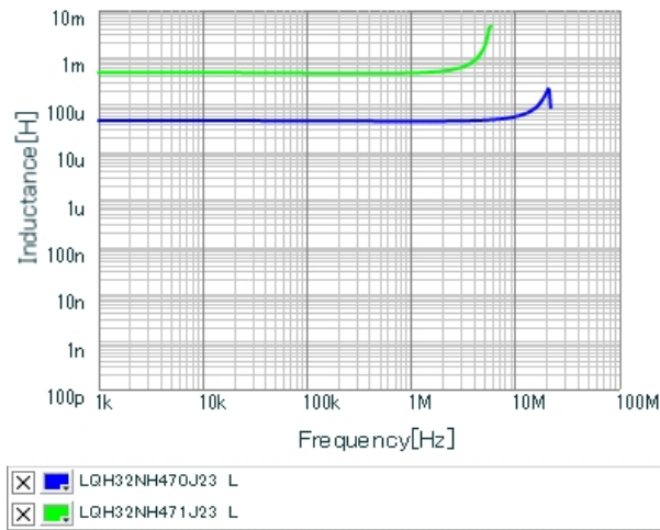
Inductance - Frequency Characteristics
