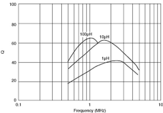
Q-Frequency Characteristics
