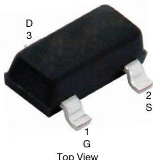
SOT-23 (TO-236)
