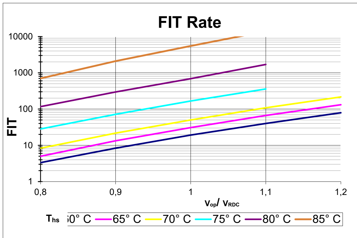
Expected Fit rate at different hot spot temperatures ( T_{hs} ) and voltage V_{RDC}
