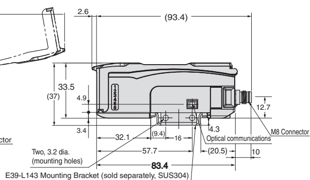
Mounting Holes
