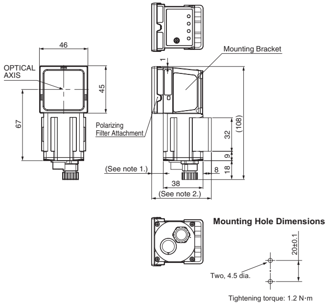
* Dimentions with the FQ-XL Mounting Bracket
