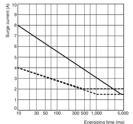
G3R-OD201SN (40 to 200 VDC)
