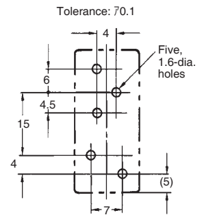
Mounting Holes
