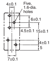
Mounting Holes
