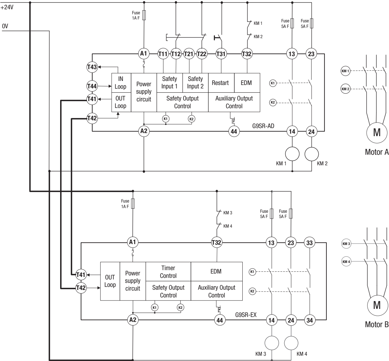
G9SR-AD with extension module G9SR-EX
