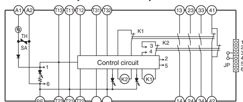
G9SA-TH301 (24 VAC/VDC)
