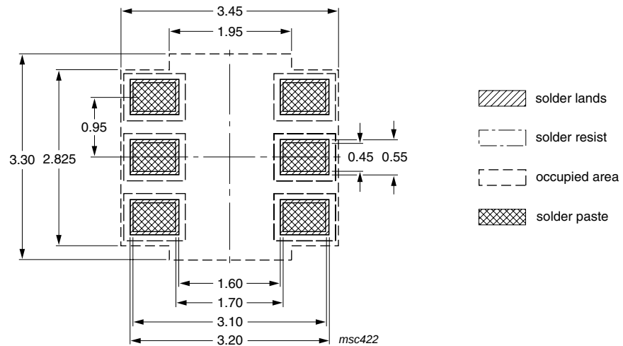
Fig 16. Reflow soldering footprint
