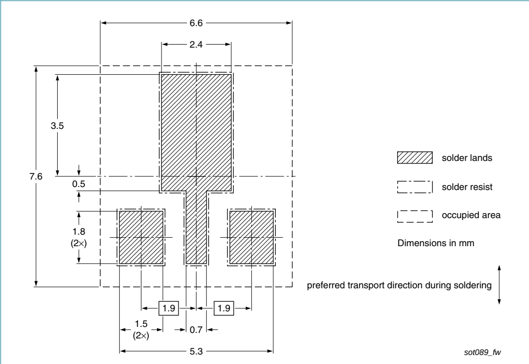
Fig 17. Wave soldering footprint SOT89 (SC-62)
