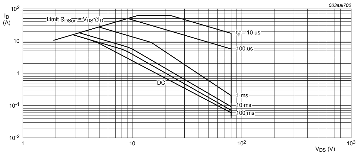
Fig. 4. Safe operating area; continuous and peak drain currents as a function of drain-source voltage T_{mb} = 25^{\circ}\text{C} ; I_{DM} is a single pulse
