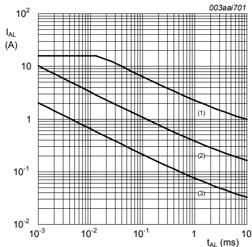
Fig. 3. Avalanche rating; avalanche current as a function of avalanche time (1) T_{j\ (init)} = 25^{\circ}\text{C} ; (2) T_{j\ (init)} = 150^{\circ}\text{C} ; (3) Repetitive Avalanche
