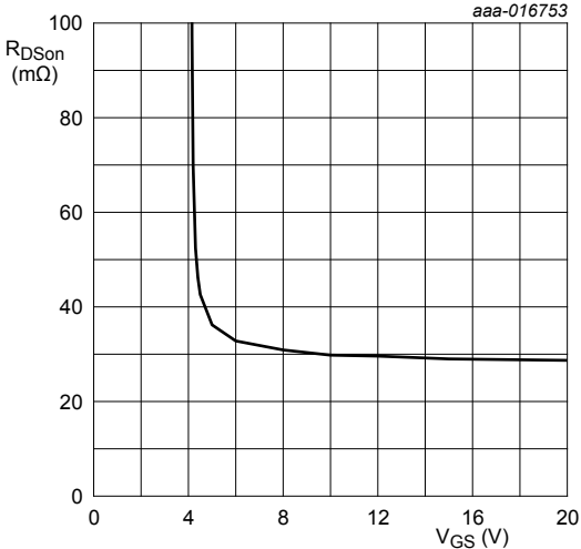
Fig. 7. Drain-source on-state resistance as a function of gate-source voltage; typical values T_j = 25^\circ\text{C}; I_D = 5\text{A}
