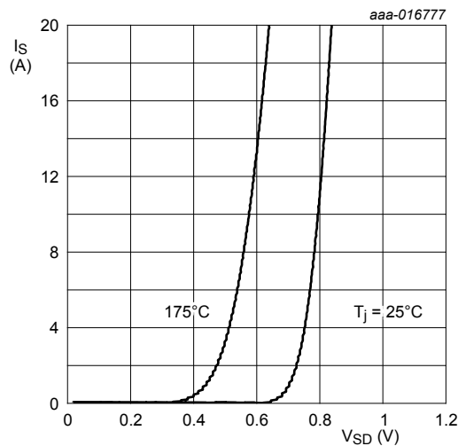
Fig. 16. Source (diode forward) current as a function of source-drain (diode forward) voltage; typical values V_{GS} = 0\text{V}
