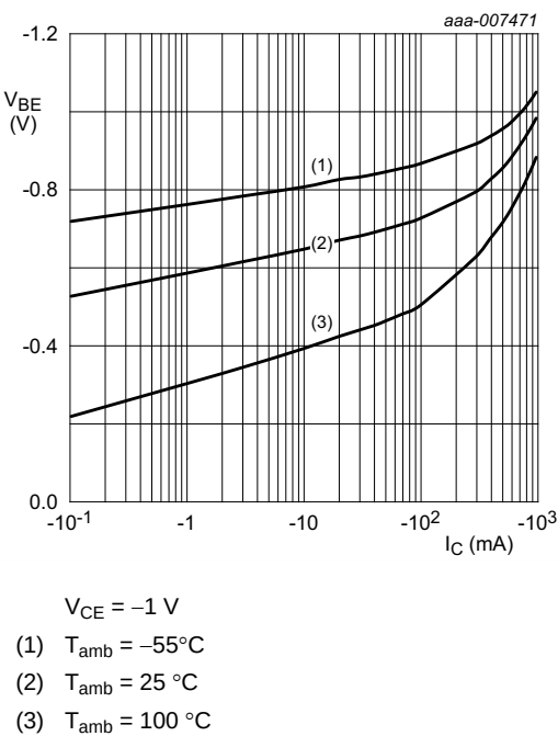
Fig 14. BC807-40QA: Base-emitter voltage as a function of collector current; typical values
