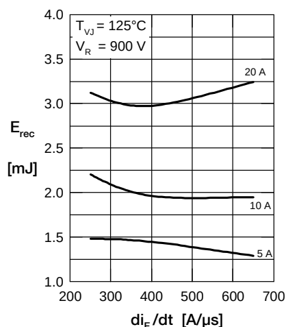
Fig. 6 Typ. recovery energy E_{rec} versus di/dt
