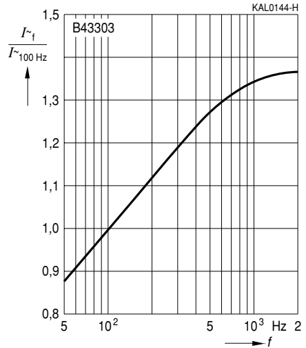
Frequency factor of permissible ripple current I_{\sim} versus frequency f U_R \geq 200 \text{ VDC}
