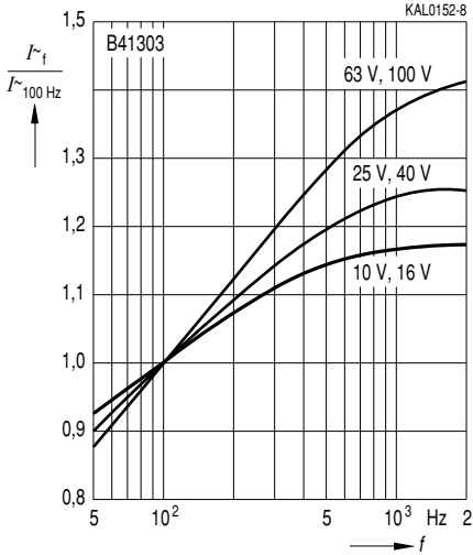
Frequency factor of permissible ripple current I_{\sim} versus frequency f U_R \leq 100 \text{ VDC}
