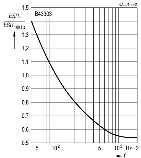
Frequency characteristics of ESR Typical behavior U_R \geq 200 \text{ VDC}
