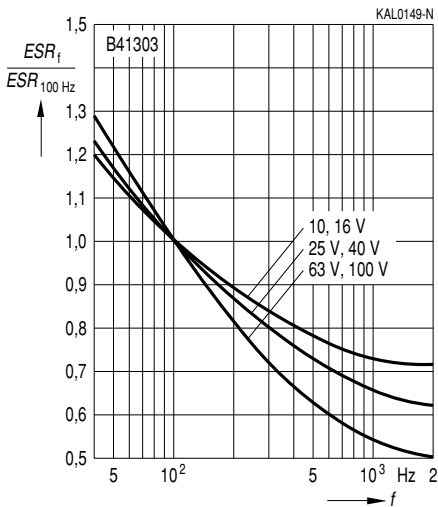
Frequency characteristics of ESR Typical behavior U_R \leq 100 \text{ VDC}
