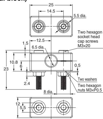
Y92E-SC06 (6.5-dia. block)
