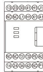
Terminal Allocations
