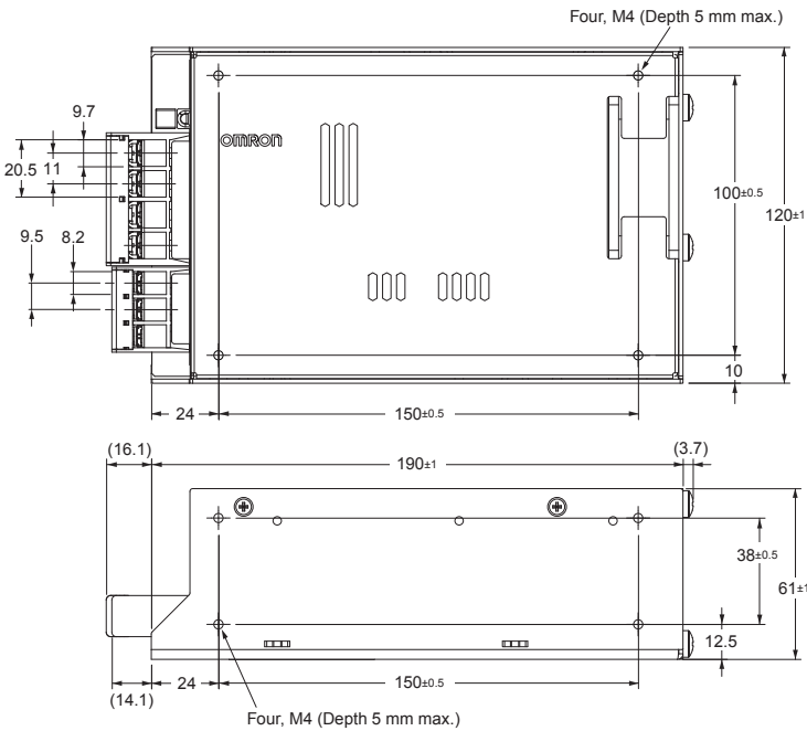
Panel mounting holes dimensions
