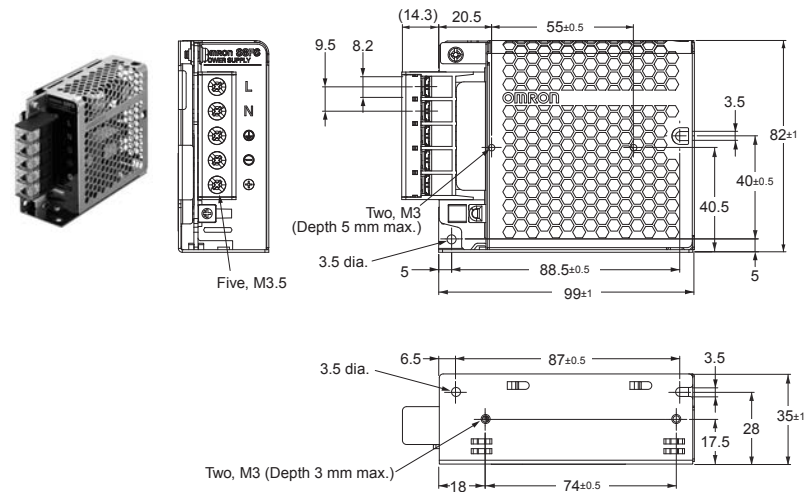
Panel mounting holes dimensions
