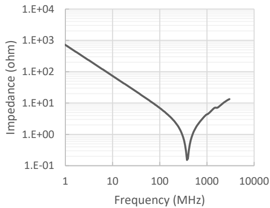
Impedance - Freq.
