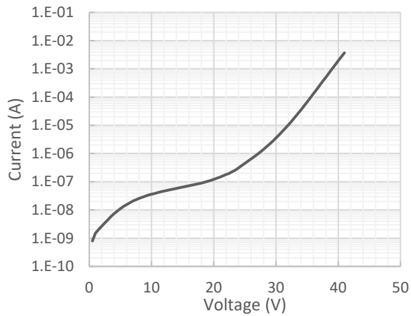
Current - Voltage
