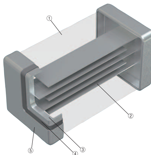
Fig.1 Internal structure of multilayer chip varistors
