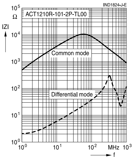
Impedance versus frequency (typical values) Current derating I_{op}/I_R ACT1210R-101-2P-TL00 versus ambient temperature
