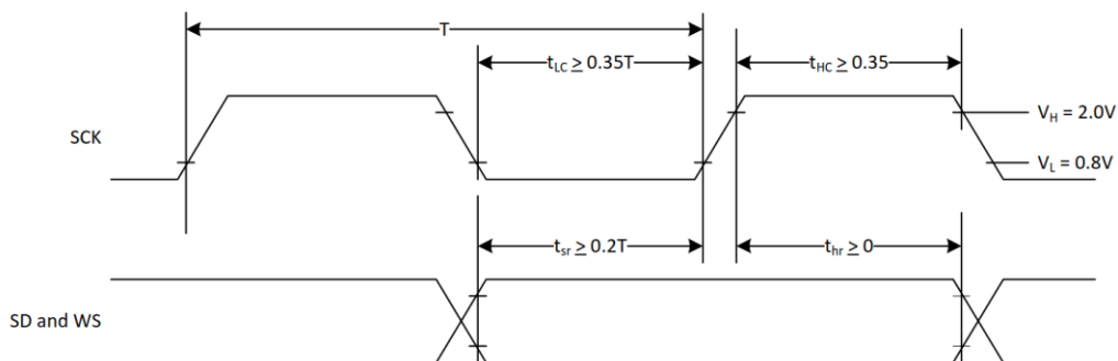
Figure 10: I²S Transmitter timing
