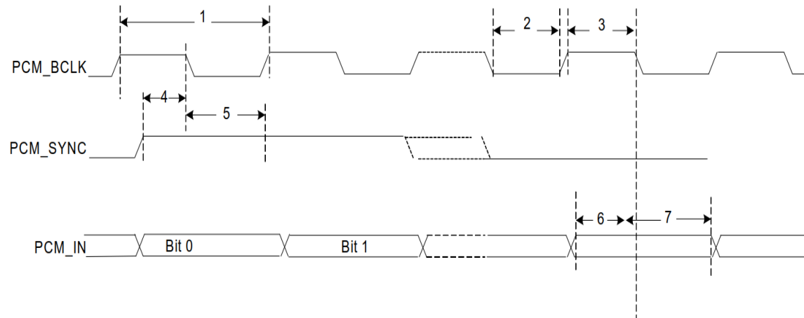
Figure 9: PCM Burst Mode Timing (Receive Only, Long Frame Sync)
