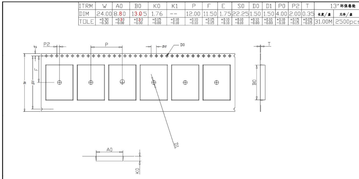
Figure 20: Tape specifications
