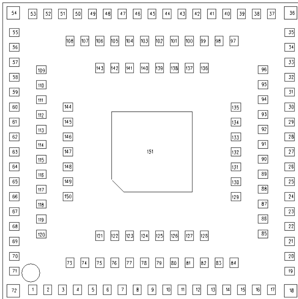
Figure 5: Sterling-EWB base SiP module pinout (top view)
