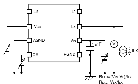
< Circuit No.⑥ >
