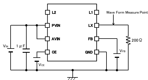
< Circuit No.③ >
