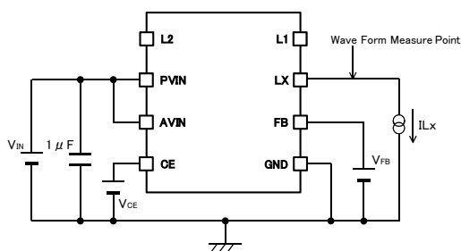
< Circuit No.④ >
