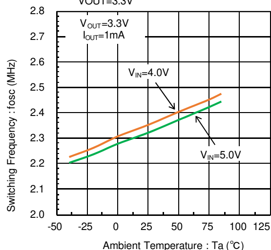
MYRGM080200X41RA V_{OUT}=3.3V
