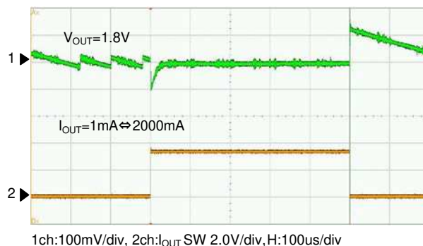
MYRGM080200C41RA V_{out}=1.8V
