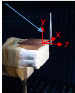
X9000984-4GDSMB in 90° bent position with 200x200 mm PCB
