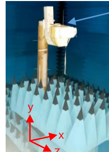
Antenna measured in Free Space
