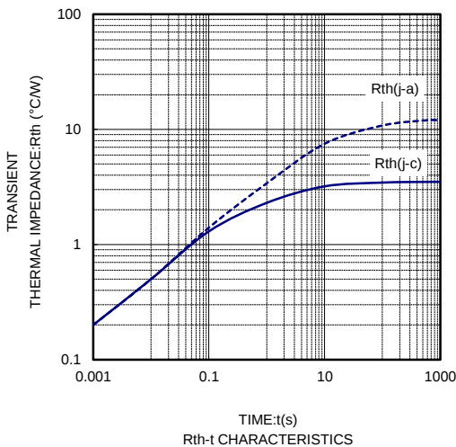
R_th-t CHARACTERISTICS
