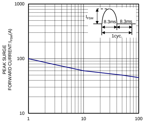
I_FSM-CYCLE CHARACTERISTICS
