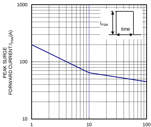
I_FSM-t CHARACTERISTICS
