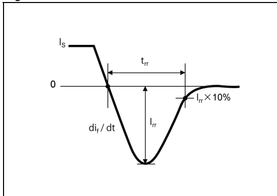
Fig.4-2 di/dt Waveform
