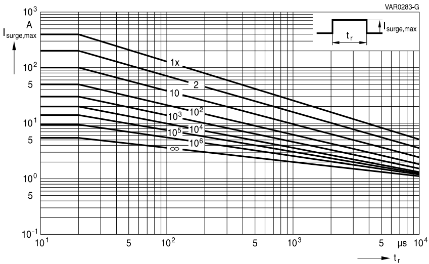
CT1210K17AUTOG_G
