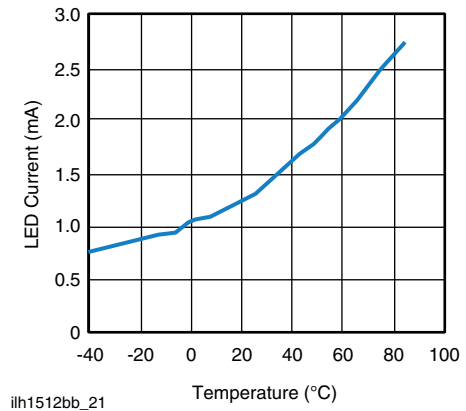
Fig. 21 - Form B Typical I_F for Switch Operation vs. Temperature
