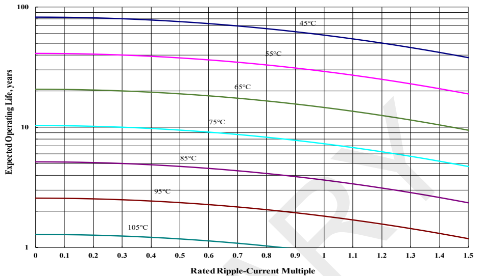
Type 381LL Operating Life in Years vs Ripple Current
