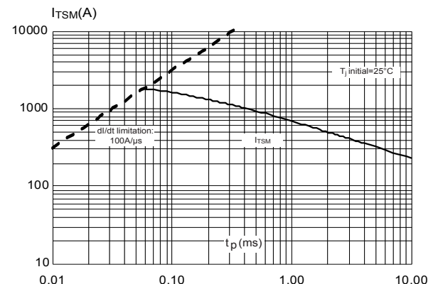
Figure 12. Non repetitive surge peak on-state current for a sinusoidal pulse with width t_p < 10 \text{ ms}
