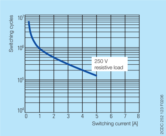
Contact lifetime
