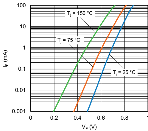
Fig. 2 - Typical Forward Current I_F vs. Forward Voltage V_F
