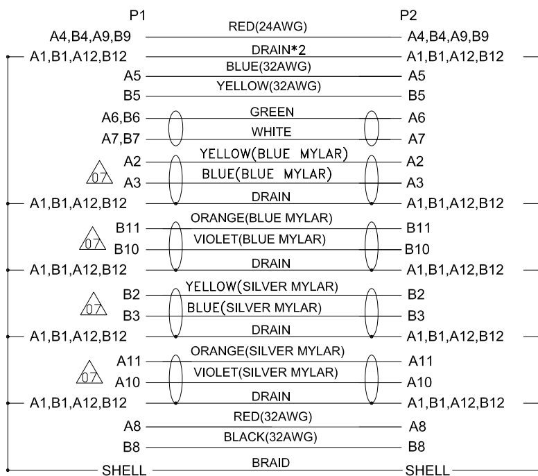
Wiring Diagram
