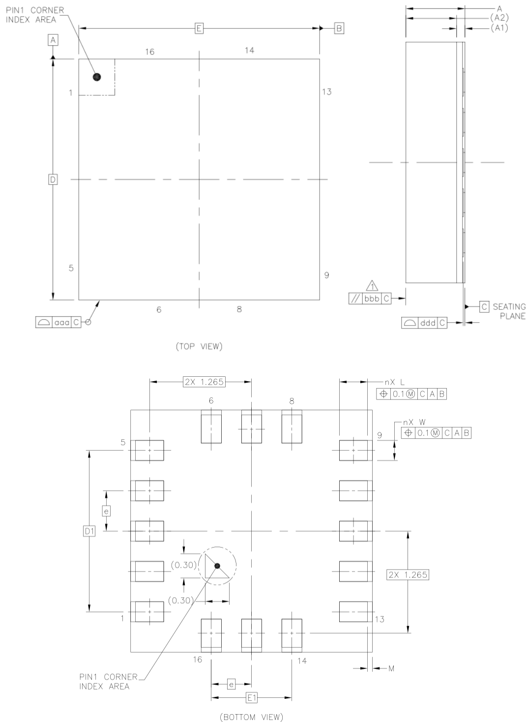
Figure 8. Package Dimensions
