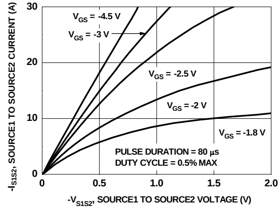
Figure 2. On-Region Characteristics
