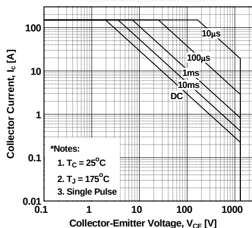
Figure 10. SOA Characteristics
