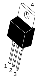
TO-220AB CASE 221A STYLE 6
