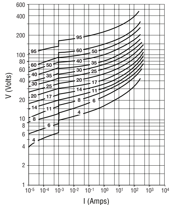
Model Size 1210 - (ZV 4 M 1210 xxx ~ ZV 95 K 1210 xxx)
