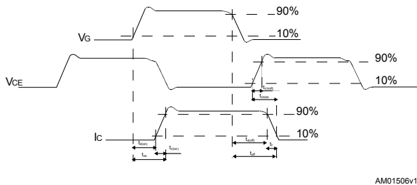
Figure 29. Switching waveform
