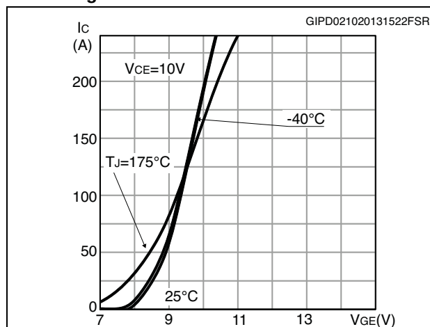
Figure 10. Transfer characteristics
