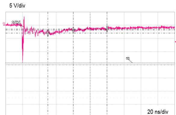
Figure 7: ESD response to IEC 61000-4-2 (-15 kV contact discharge)
