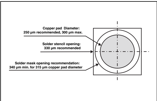
Figure 14. Footprint
