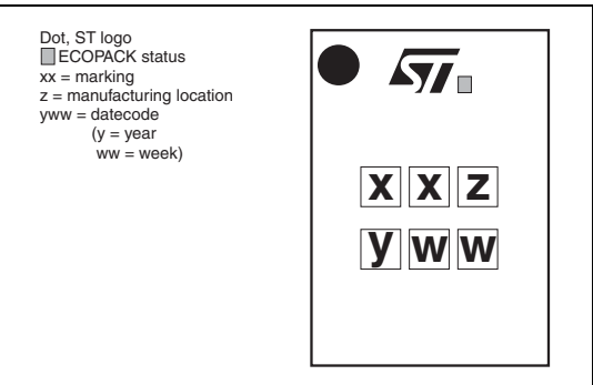
Figure 15. Marking
